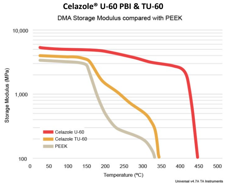
Figure 2 - DMA Curve Source: PBI Performance Products
