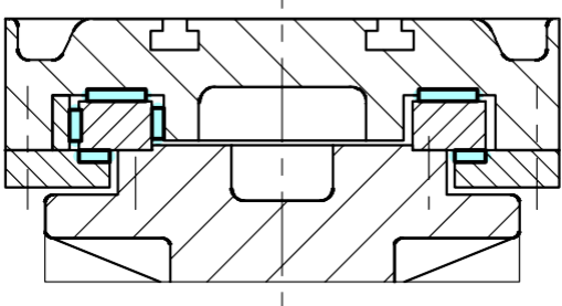
Flat Guideway
