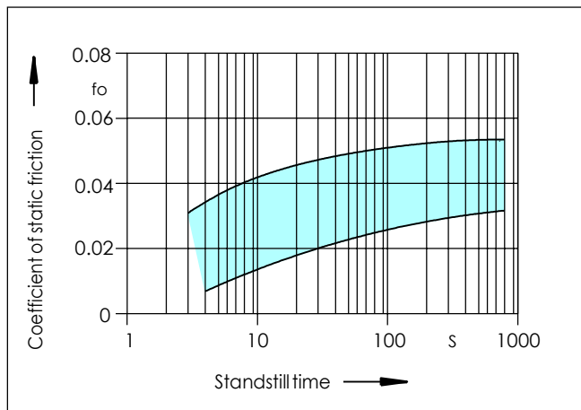
Figure 5 Range of the coefficient of static friction ( f_0 ) as a function of the standstill time when using different lubricants
