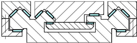
Double V-Guideway
