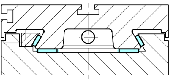
Dovetail Guideway
