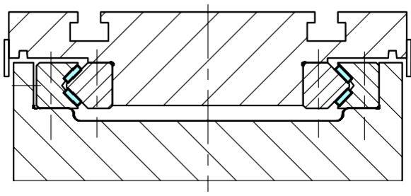
V-Guideway
