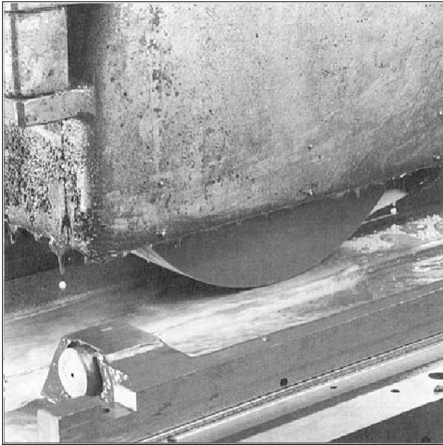
Figure 10 Grinding
