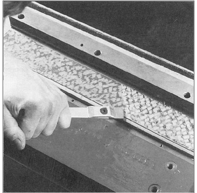
Figure 11 Scraping
