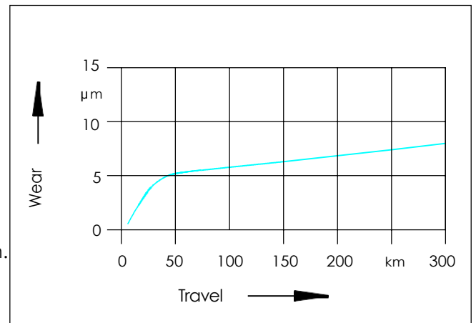
Figure 8 Wear behaviour of Turcite-B Slydway®
